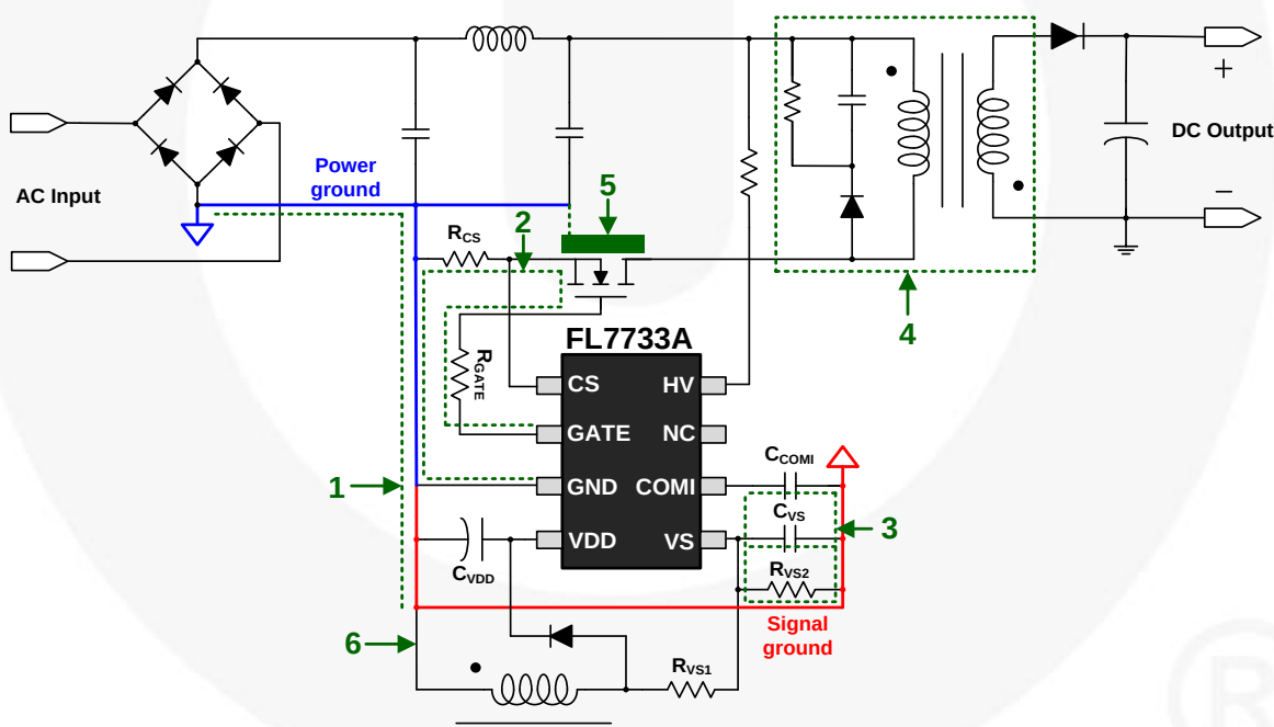
Figure 28. Layout Example
